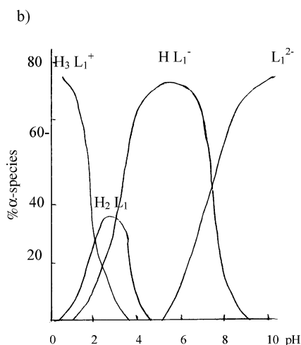
FIGURE 2 pH-species distribution profile for L_1 species.
