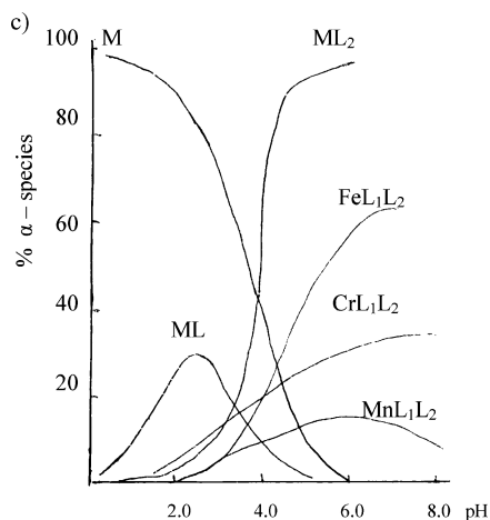
FIGURE 3 pH-species distribution profile for the Binary and ternary M:L_1:L_2 systems.
